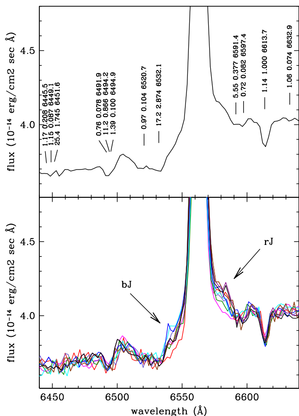
Figure 16. Top panel: average around H\alpha of the low-resolution spectra of VES 263. The strongest DIBs in the compilation by Jenniskens & Desert (1994) are marked (see Section 8.4 for associated numbers). Bottom panel: the individual spectra making up the above average are plotted individually (after matching their median value). The arrows point to regions at \approx -700 and +700 km s^{-1} where the dispersion is larger (see section 7.4).
