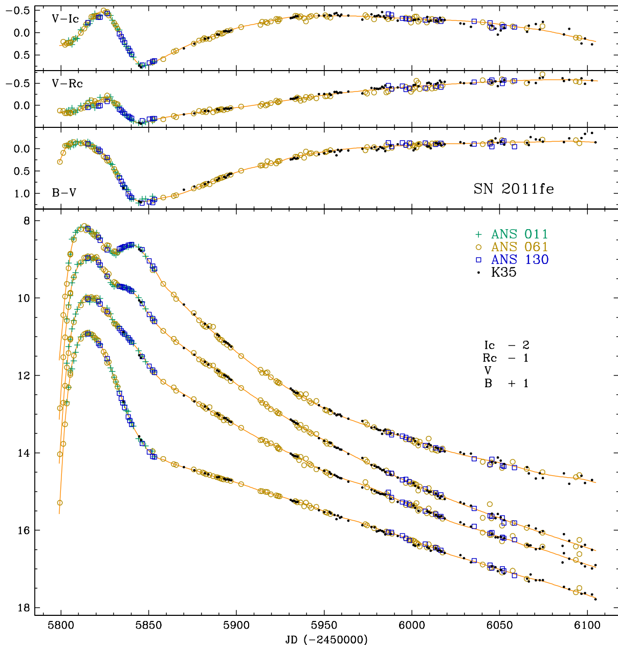
Figure 3: BVRcIc light- and color-curve of SN 2011fe from our data in Table 1. Different colors and symbols identify the telescopes used to monitor the supernova. The curves are spline fits to the data drawn to guide the eye.
