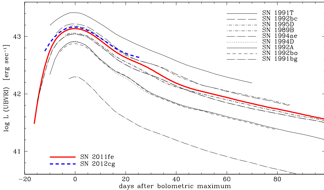
Figure 4: Bolometric lightcurves of SN 2011fe and SN 2012cg (obtained by summing the reddening corrected flux in the UBVRCIC bands) compared to those of well observed objects from Contardo et al. (2000). The U data are obtained from observed B values and adding the parametrized U-B color evolution from Nobili and Goobar (2008).
