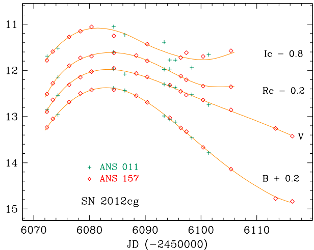
Figure 6: BVR_C I_C lightcurve of SN 2012cg from our data in Table 2. Different colors and symbols identify the telescopes used to monitor the supernova. The curves are spline fits to the data drawn to guide the eye.
