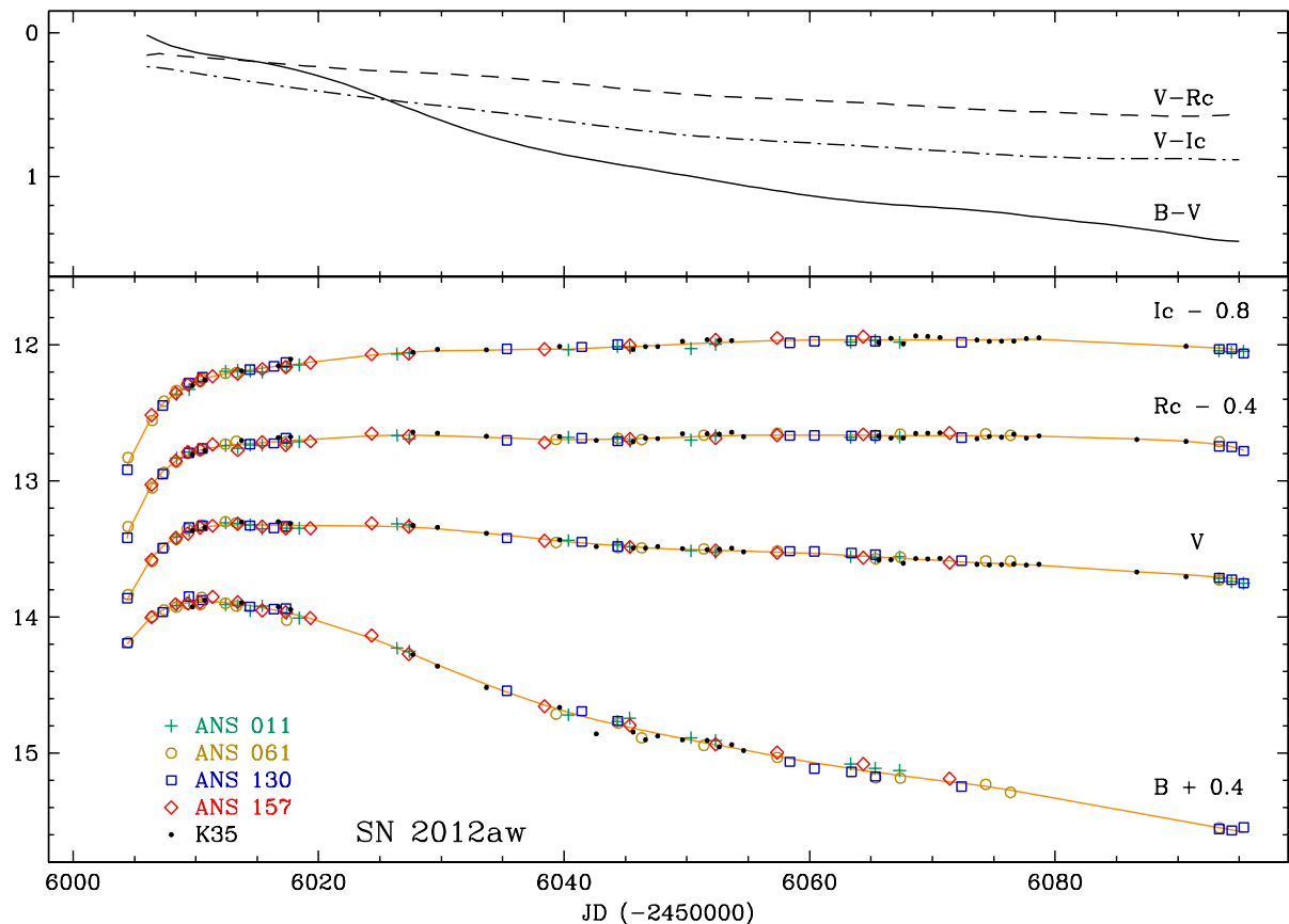
Figure 7: BVRcIc light- and color-curves of SN 2012aw from our data in Table 3. Different colors and symbols identify the telescopes used to monitor the supernova. The curves are spline fits to the data drawn to guide the eye.
