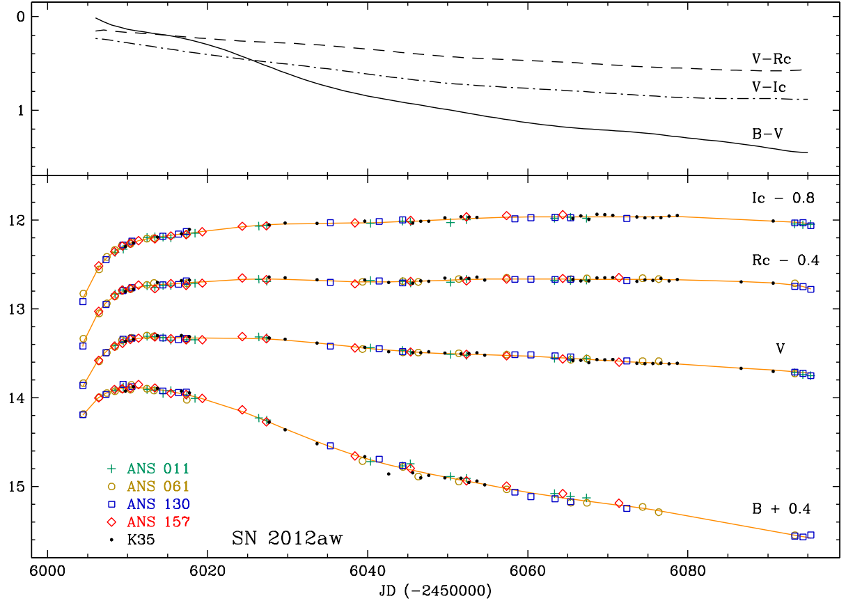
Figure 7: BVR_CI_C light- and color-curve of SN 2012aw from our data in Table 3. Different colors and symbols identify the telescopes used to monitor the supernova. The curves are spline fits to the data drawn to guide the eye.
