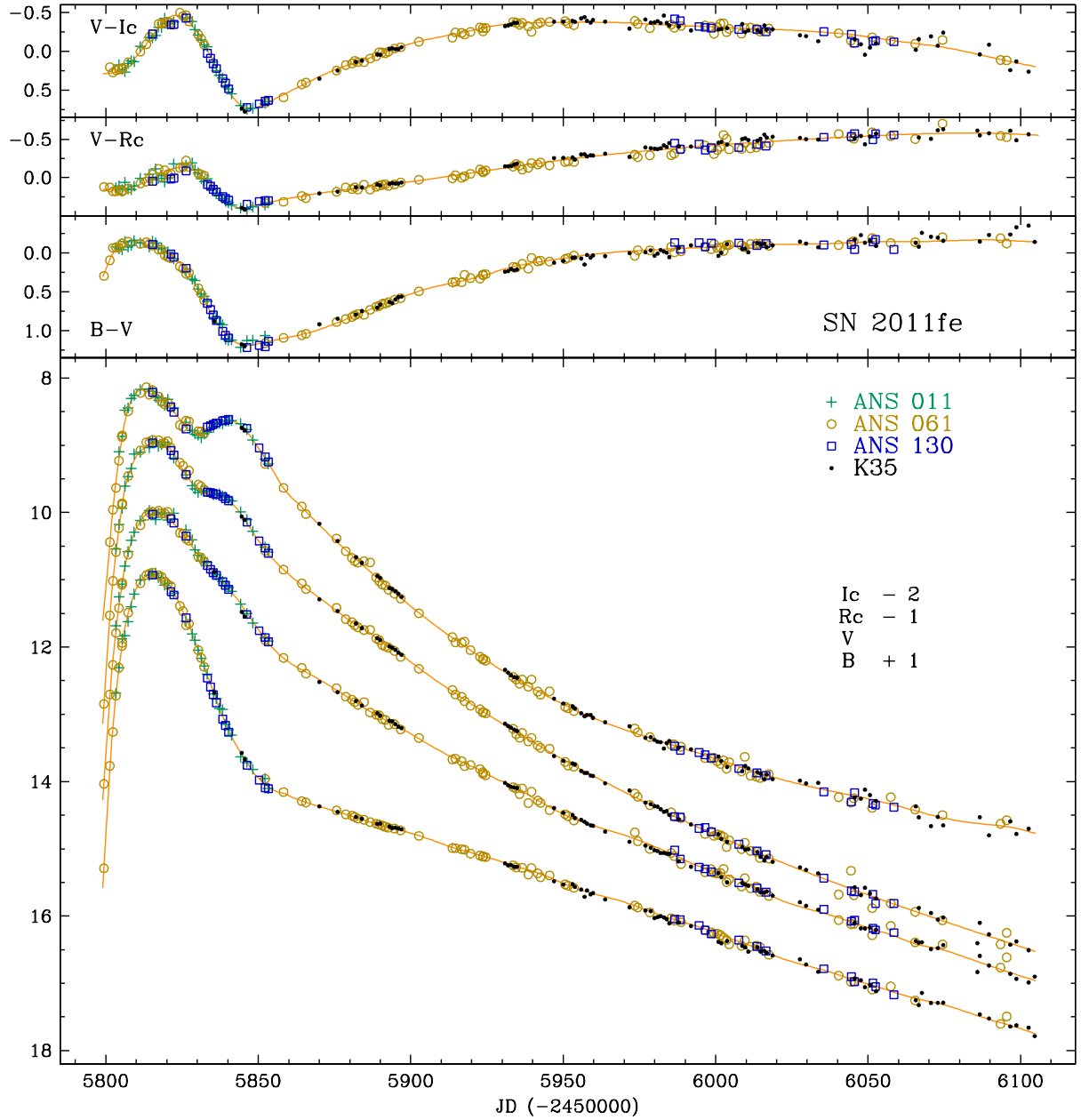
Figure 3: BVR_{CI} light- and color-curve of SN 2011fe from our data in Table 1. Different colors and symbols identify the telescopes used to monitor the supernova. The curves are spline fits to the data drawn to guide the eye.
