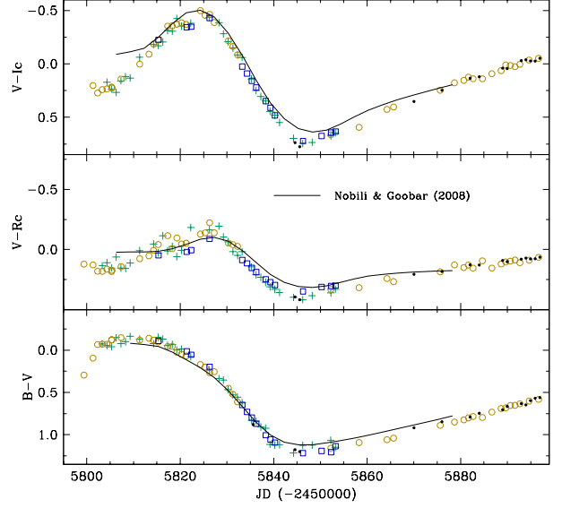
Figure 5: Comparison of the color evolution of SN 2011fe with the parameterized color evolution of Nobili and Goobar (2008), over-plotted as a curve.
