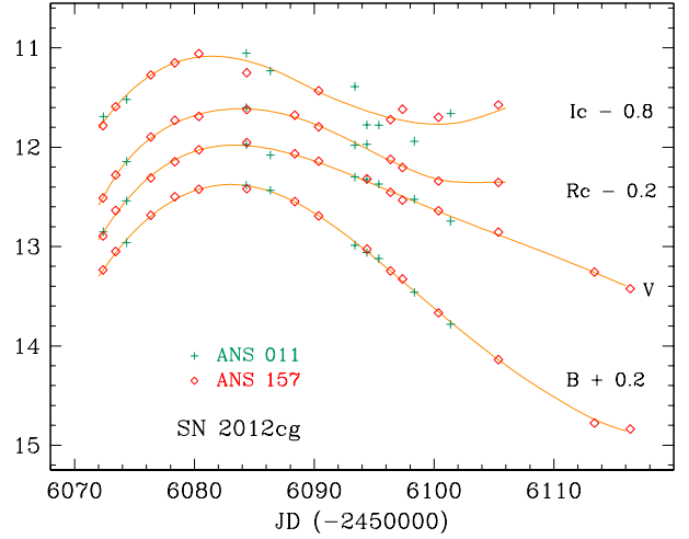
Figure 6: BVR_CI_C lightcurve of SN 2012cg from our data in Table 2. Different colors and symbols identify the telescopes used to monitor the supernova. The curves are spline fits to the data drawn to guide the eye.
