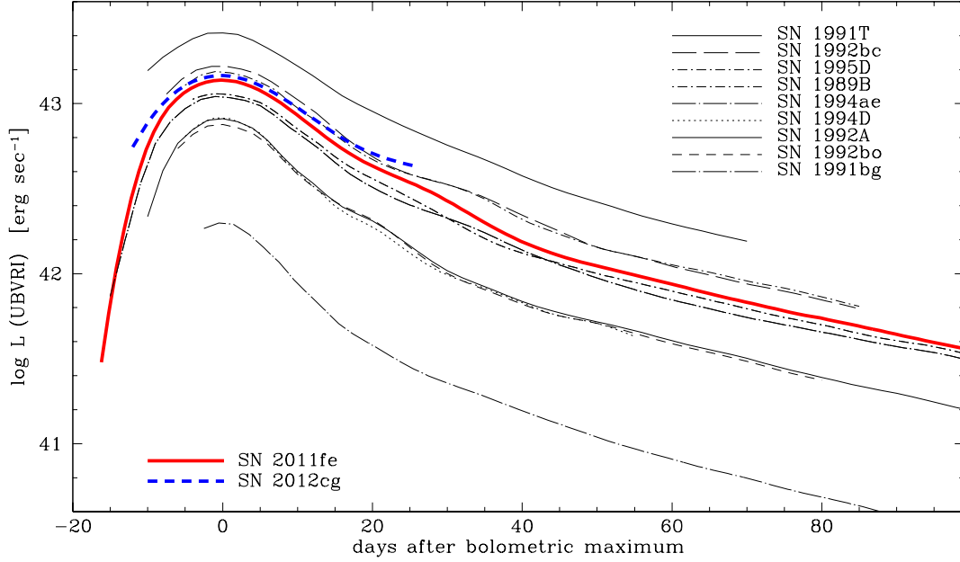
Figure 4: Bolometric lightcurves of SN 2011fe and SN 2012cg (obtained by summing the reddening corrected flux in the UBVR_CI_C bands) compared to those of well observed objects from Contardo et al. (2000). The U data are obtained from observed B values and adding the parametrized U-B color evolution from Nobili and Goobar (2008).
