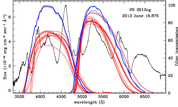
Figure 1: A spectrum of SN 2012cg with overplotted the measured transmission profiles of many B and V filters from different manufacturers (from Munari and Moretti 2012). Red curves refer to common filters made with sandwiches of colored glasses, blue curves to multi-layer dielectric filters. The different amount of transmitted absorption and emission features is evident (especially on the red wing of V filter passband), which account for the unavoidable differences in the photometry obtained with different telescopes even if a given SN is measured against the same identical photometric sequence.
