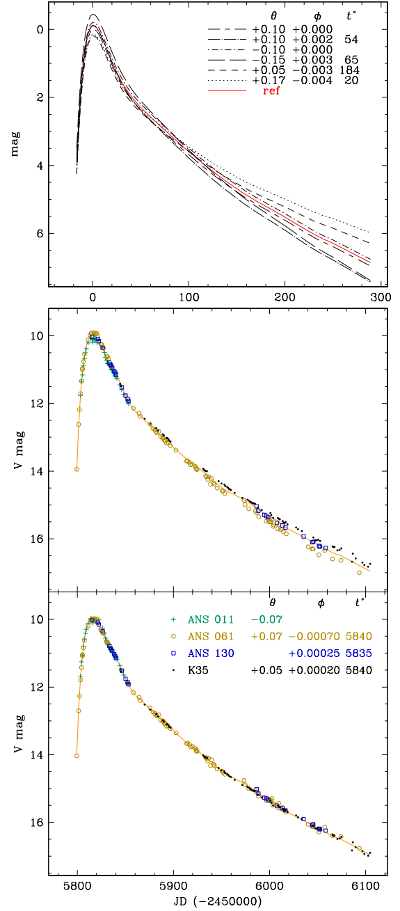
Figure 2: Example of the lightcurve merging method (LMM) described in Sect. 3. Top : These lightcurves are the results of shifting (by \theta ) and stretching (by \phi ) around the pivot points ( t^* ) the ordinates (magnitudes) of the reference lighthcurve (plotted in red). Middle : our source V -band observations for SN 2011fe, where different colors and symbols identify different telescopes. Bottom : our merged V -band lightcurve of SN 2011fe after application (by the given quantities) of the LMM shift and pivot stretching method. The orange line (the same in both the middle and bottom panels) is a spline fit to the merged lightcurve \text{mag}(\lambda)_{i,j} (cf. Eq.(3)).
